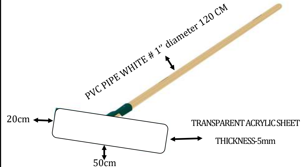
Plane Rake- Customized design of Acrylic Sheet, thickness 5mm and PVC pipe #1"
