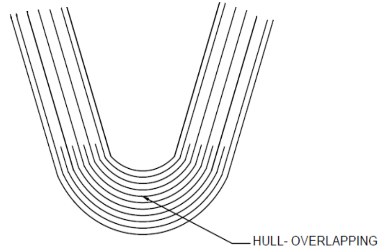
MIDSHIP SECTION LAMINATION DETAILS
