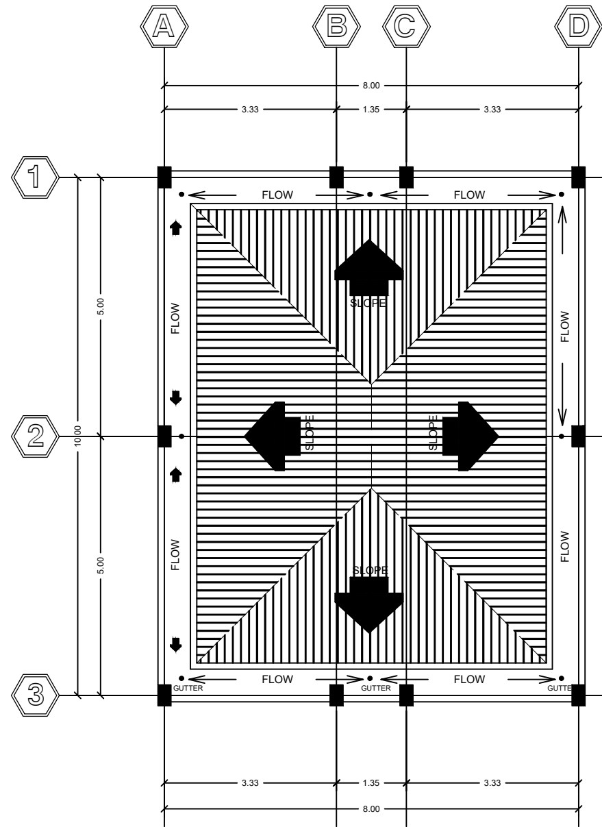
A ROOF PLAN 3/7 SCALE 1:100 mts
