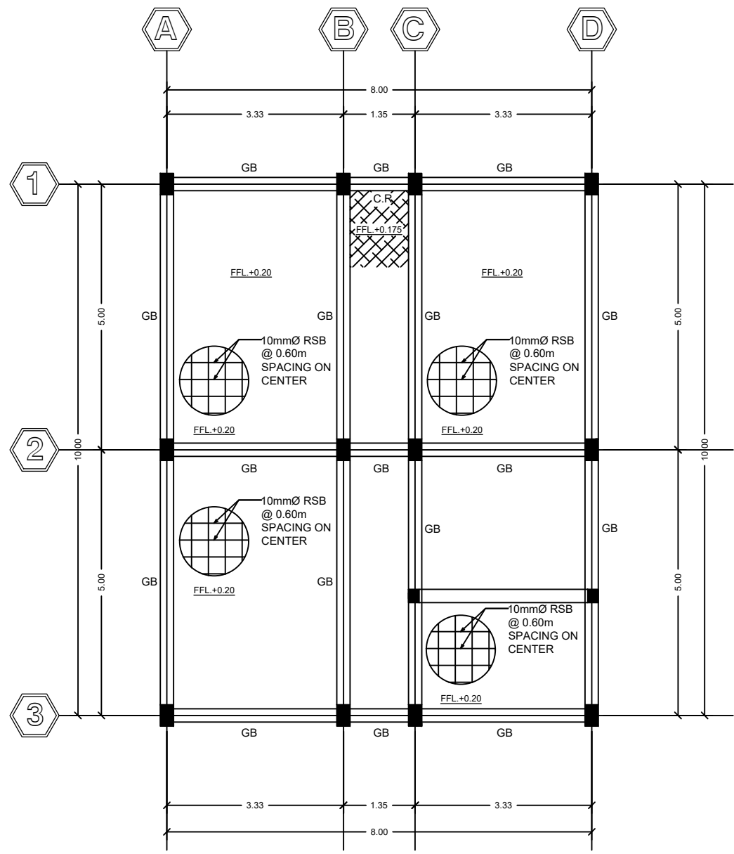
S 3/6 GRADE BEAM LAYOUT SCALE 1:100 mts
