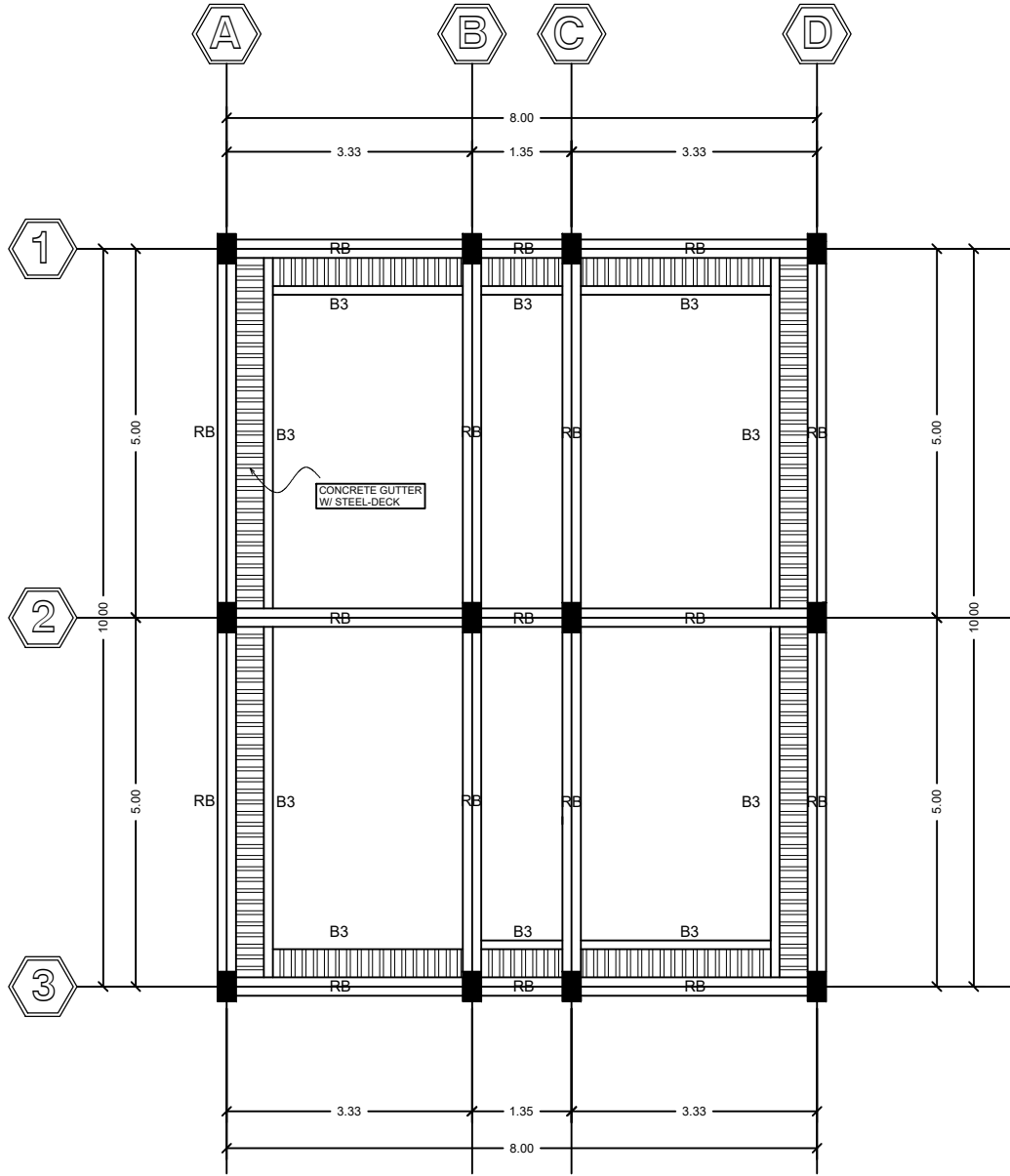
S 46 SCALE 1:100 mts ROOF BEAM LAYOUT
