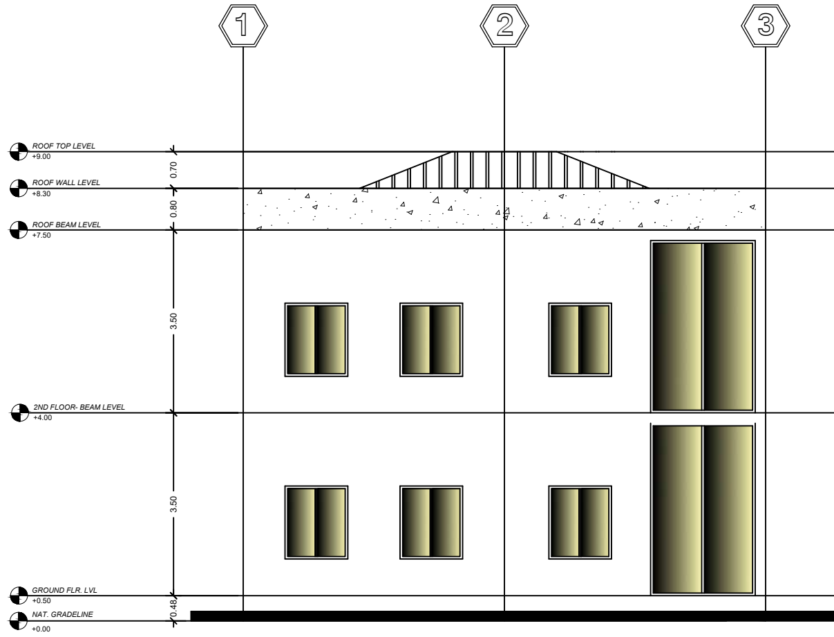
A 67 LEFT-SIDE ELEVATION SCALE 1:100 mts
