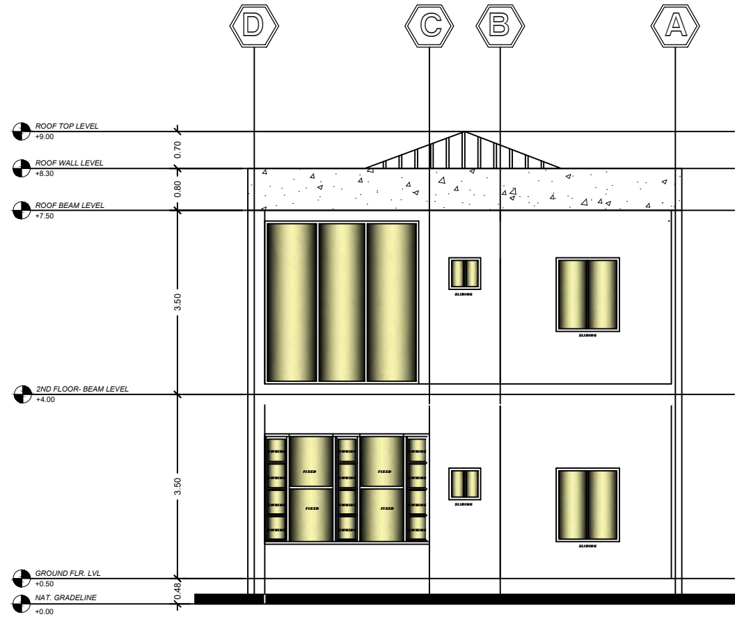
A REAR ELEVATION 5/7 SCALE 1:100 mts
