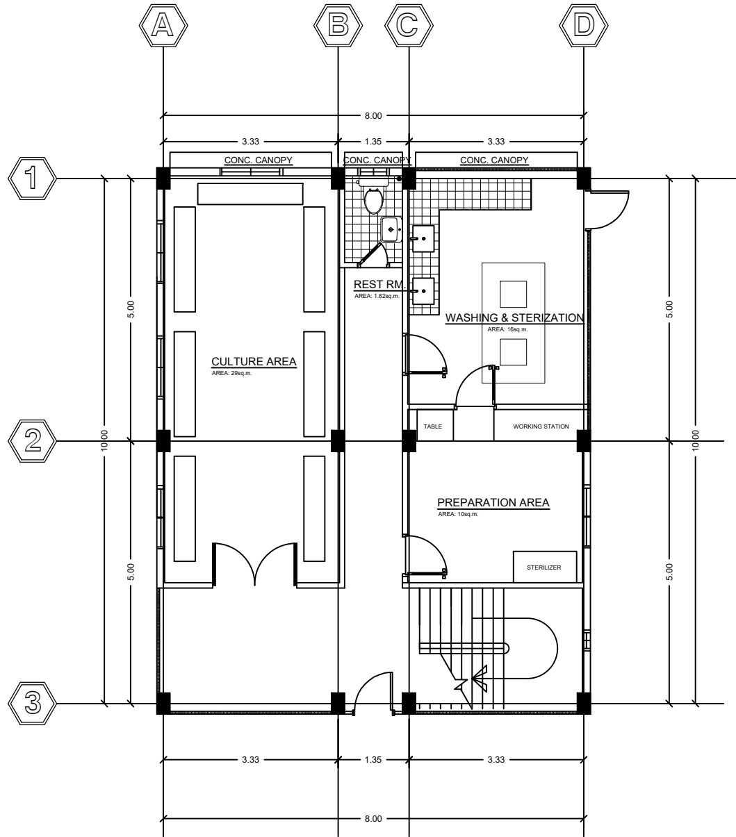
A 17 GROUND FLOOR PLAN SCALE 1:100 mts
