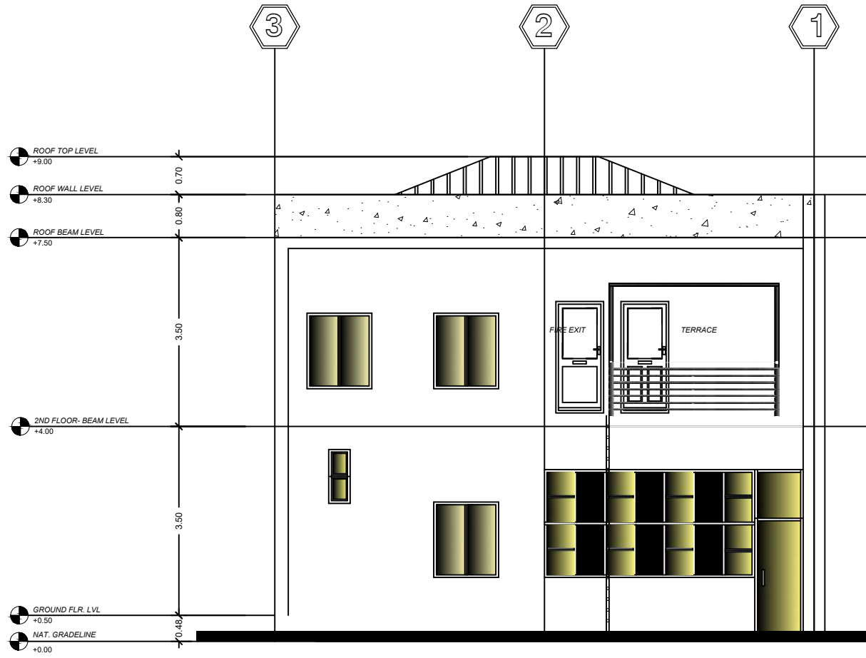
A RIGHT-SIDE ELEVATION 7/7 SCALE 1:100 mts
