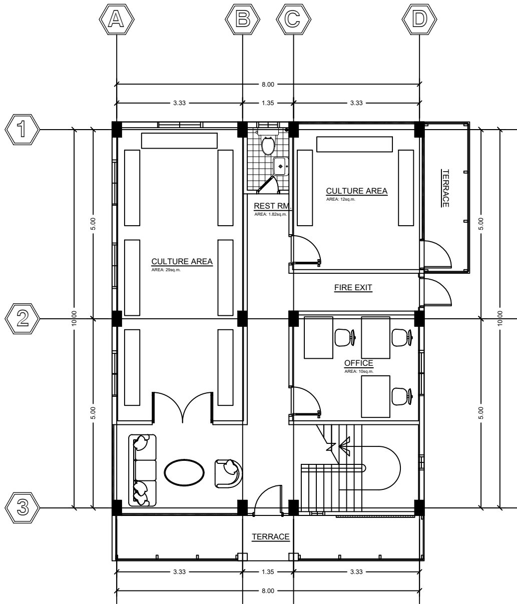
A 2ND FLOOR PLAN 2/7 SCALE 1:100 mts
