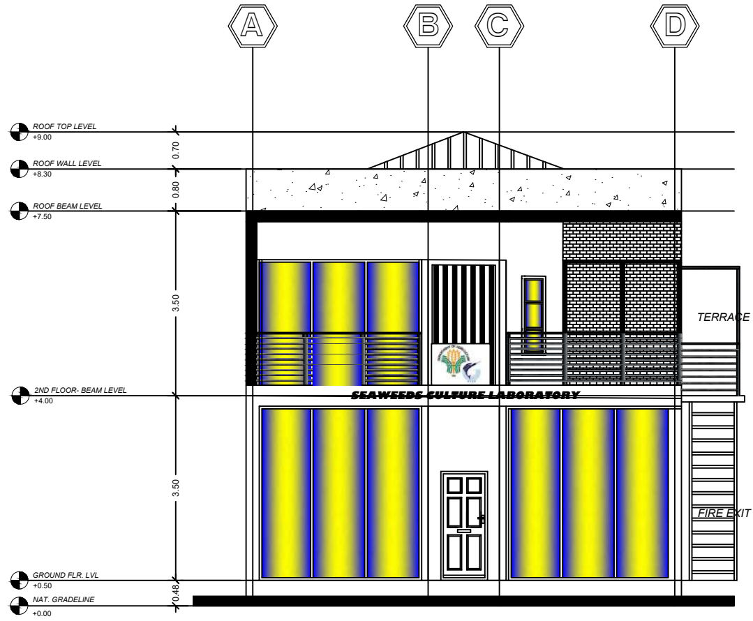
A 47 FRONT ELEVATION SCALE 1:100 mts
